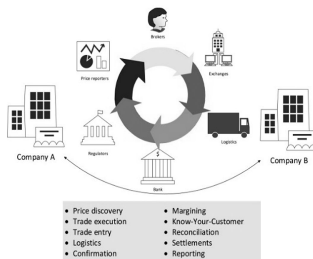
Fig. 3.2 Blockchain Technology.
